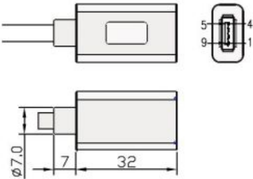
USB 3.0 A female
