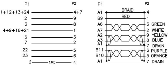
PINOUT
