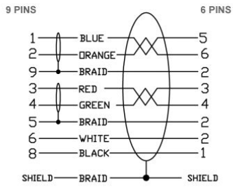
PINOUT 9 TO 6 FIREWIRE CABLE
