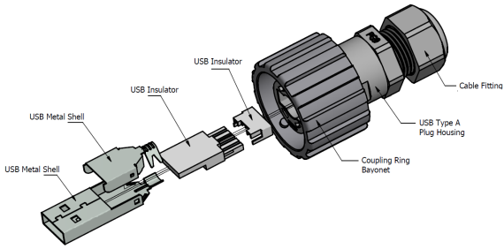
USB 2.0 male
