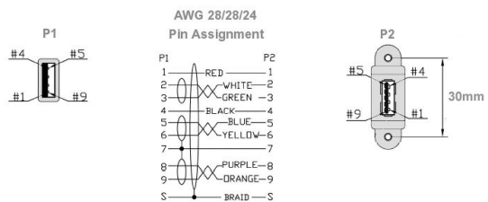
USB 3.0 A
