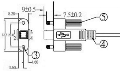
USB 2.0 B plug A110-507-001
